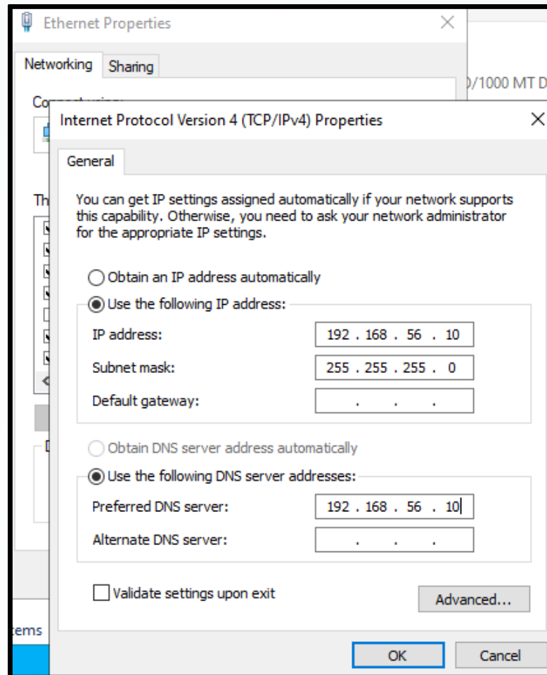
Figure 3. Configuring a static IP address and verifying the network configuration using ipconfig.
